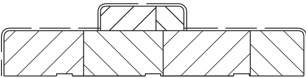
DJ-01 Double Rabbet Jamb
