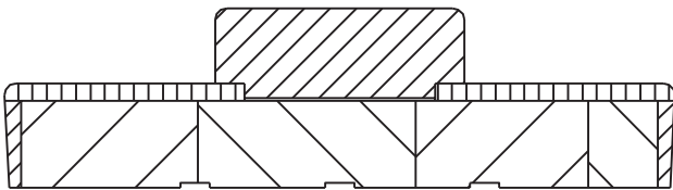
DJ-01 Double Rabbet Jamb
